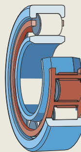
Hybrid cylindrical roller bearing
