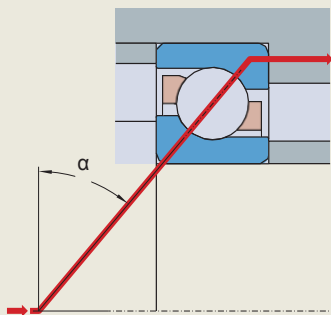
Fig. 1 Contact angle \alpha - load transmission
