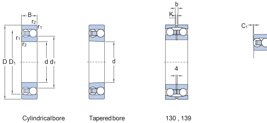
Cylindrical bore
