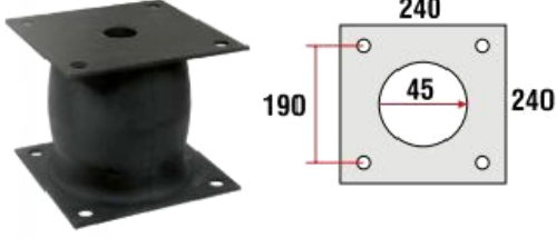
240'LİK ELEK TAKOZU / 240 Ø BUFFERS
