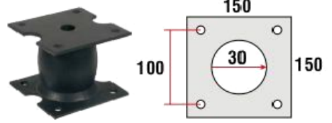
150'LİK ELEK TAKOZU / 150 Ø BUFFERS
