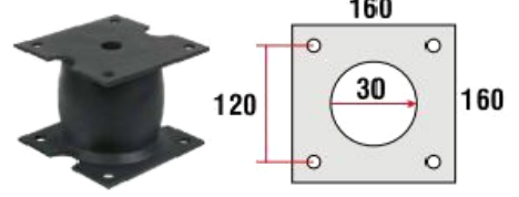
150'LİK ELEK TAKOZU / 150 Ø BUFFERS
