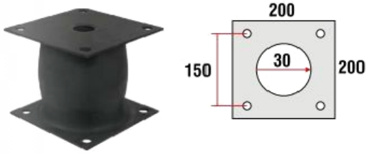
200'LİK ELEK TAKOZU / 200 Ø BUFFERS
